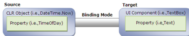
Figure 5.1 A conceptual view of data binding.
