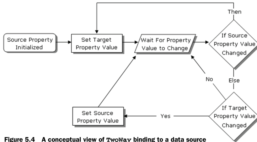
Figure 5.4 A conceptual view of TwoWay binding to a data source
