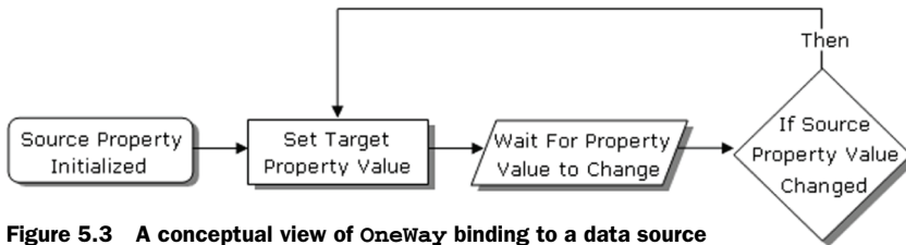
Figure 5.3 A conceptual view of OneWay binding to a data source
