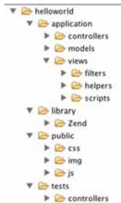
Figure 2.2 A typical Zend Framework application's directory layout groups the files by their role in the application, so it is easy to find the file you are looking for.
